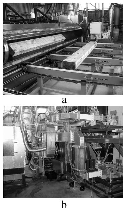
Figure 1.—A 300-kW MW plant (frequency, 0.922 GHz) for large cross-section round and sawn timber modification: (a) general view from the out-feed side; (b) four-port MW applicator with waveguides for MW power supply to the applicator from generators.
